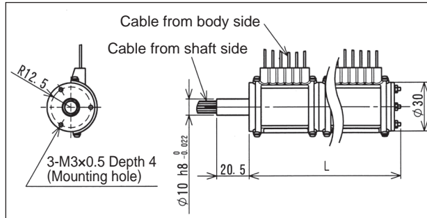
SRP-300318S (14~18 poles)
