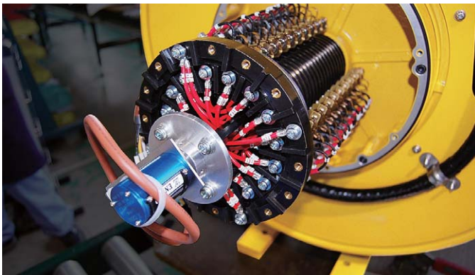
AC600V-20A-30P+SRP-CL4
