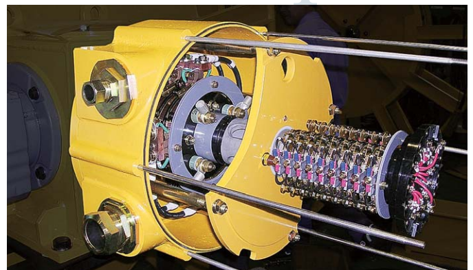
AC600V-20A-8P+SPM-50-16P-02
