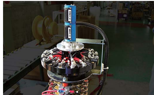
AC600V-30A-8P+10A-20P+SRP-300312S
